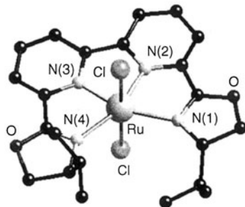
Fig. 62. Molecular structure of [RuCl 2 (48)] (R = i -Pr).
