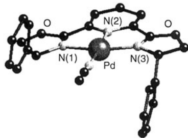
Fig. 56. Molecular structure of [\text{Pd}(\text{CH}_3\text{CN})(\mathbf{42})][\text{BF}_4]_2 ( R = \text{Ph} ). The tetrafluoroborate anions have been omitted for clarity.
