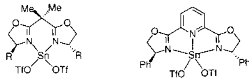
Fig. 66. Tetra- and pentacoordinated tin complexes.
