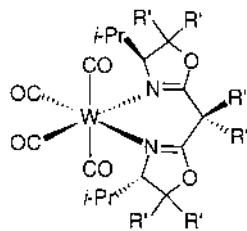
\mathbf{36} , \text{R}' = \text{H} \mathbf{37} , \text{R}' = \text{Me}
