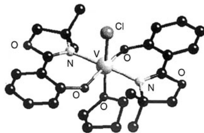
Fig. 19. Molecular structure of [\text{VCl}(\mathbf{13})_2(\text{THF})] ( X = Y = R'' = \text{H} , R = R' = \text{Me} ).
