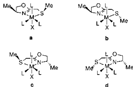
Fig. 23. Diastereomers for the fac -[MXL 3 (17)] complexes.
