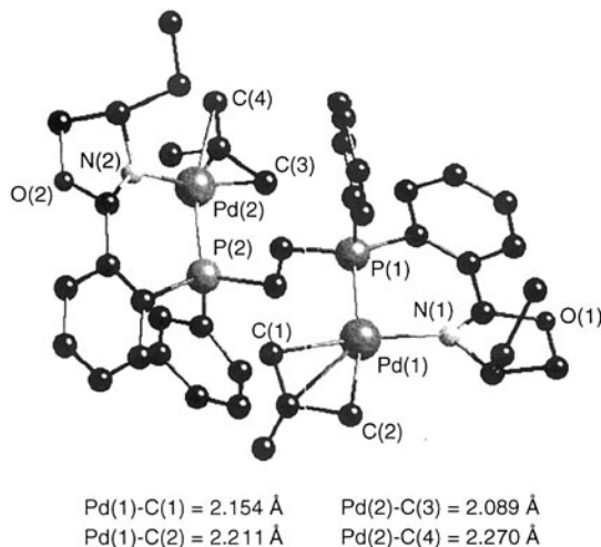
Fig. 65. Molecular structure of [\text{Pd}_2(\eta^3\text{-2-Me-C}_3\text{H}_4)_2(\mu\text{-N}_2\text{P}_2)](\text{PF}_6)_2 . The hexafluorophosphate anions have been omitted for clarity.
