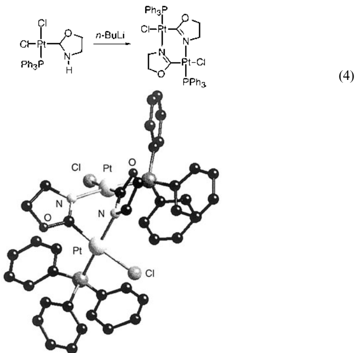
Fig. 4. Molecular structure of [PtCl(PPh 3 ){μ-COCH 2 CH 2 N–C,N}] 2 .
