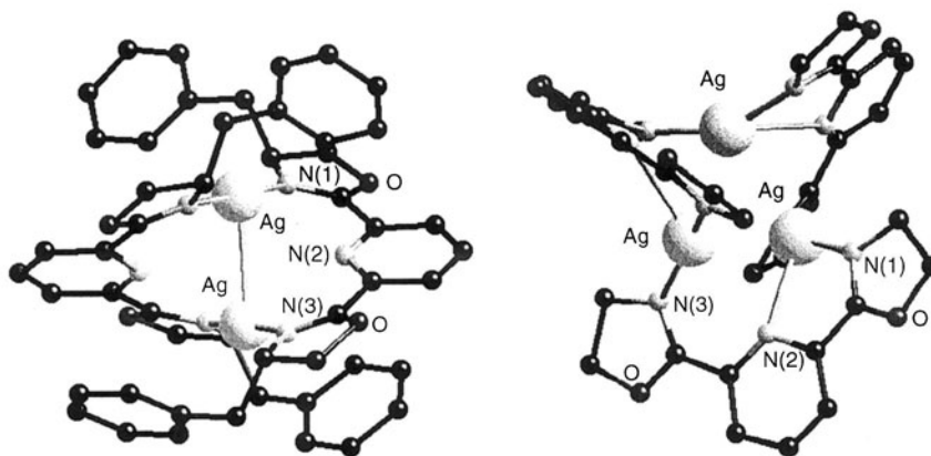
Fig. 57. Molecular structure of [\text{Ag}_2(\mathbf{42})_2](\text{BF}_4)_2 and [\text{Ag}_3(\mathbf{42})_3](\text{BF}_4)_3 , R = \text{Ph} complexes. The phenyl substituents on oxazoline moieties and tetrafluoroborate anions have been omitted for clarity.
