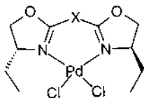
Fig. 70. Model of the palladium structure used for geometrical calculations.
