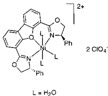
Fig. 59. Hexacoordinated Ni(II) complex with terdentate 47 ligand.
