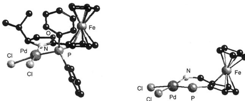
Fig. 34. Molecular structure of [\text{PdCl}_2(\text{S},\text{S}\text{-}\mathbf{30})] and the detail of the Pd coordination sphere.
