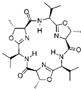
Fig. 60. Free cyclopeptide ligand.
