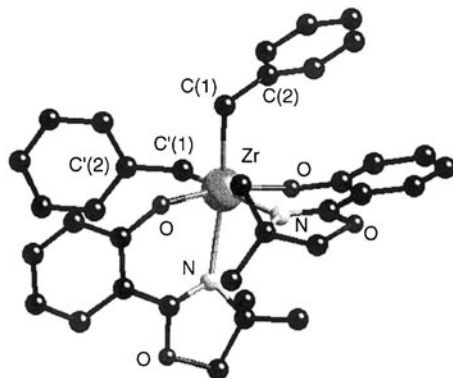
Fig. 20. Molecular structure of cis - [\text{Zr}(\text{CH}_2\text{Ph})_2(\mathbf{13})_2] ( X = Y = R'' = \text{H} , R = R' = \text{Me} ).
