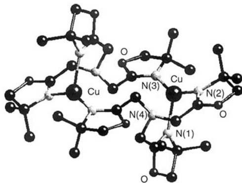
Fig. 58. Molecular structure of [\text{Cu}(\mathbf{44})]_2(\text{BF}_4)_2 . The tetrafluoroborate anions have been omitted for clarity.
