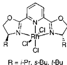
Fig. 54. Rhodium precursors in the hydrosilylation on ketones.
