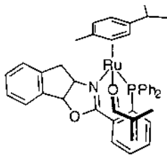
Fig. 25. Proposed intermediate in the Diels–Alder reaction [67].
